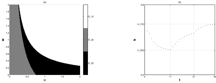
Figure 2: (a) Long run equilibrium points for system T when varying w and \alpha given the following values of the other parameters: n = 1 , s = 0.2 , \tau = 0.3 , \rho = 0.5 , \delta = 0.2 , A_l = 5 , A_h = 6 , c^h = 0.8 , c^l = 0.1 and p = 1 . The initial condition is m_0 = 0.5 and k_0 = 0.5 . (b) Trajectory of the system for initial condition and parameter values as in (a) while w = 0.2 for t = 1, 2, \dots, 10 , w = 0.9 for t = 11, 12, \dots, 20 and w = 1.6 for t = 21, 22, \dots, 30 .
